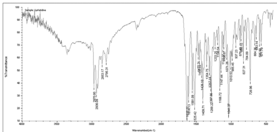
Figure 4: IR spectrum of Lafutidine + gellan gum + HPMC K100 M physical mixture.
