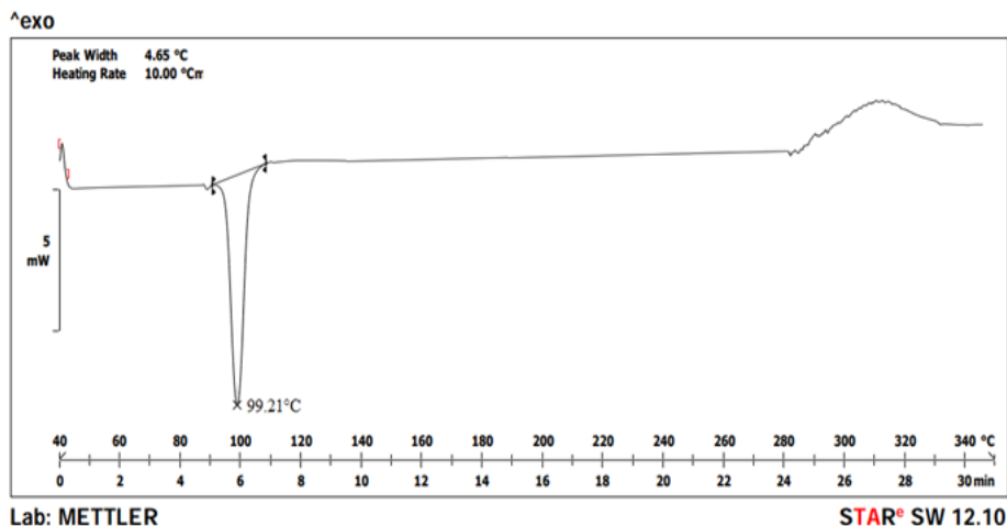
Figure 2: DSC thermogram of Lafutidine.
