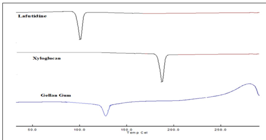
Figure 5: DSC thermogram of Lafutidine, Xyloglucan and gellan gum
